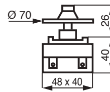
Bare model P/N. 9014-01 (weight 0,11 kg).
